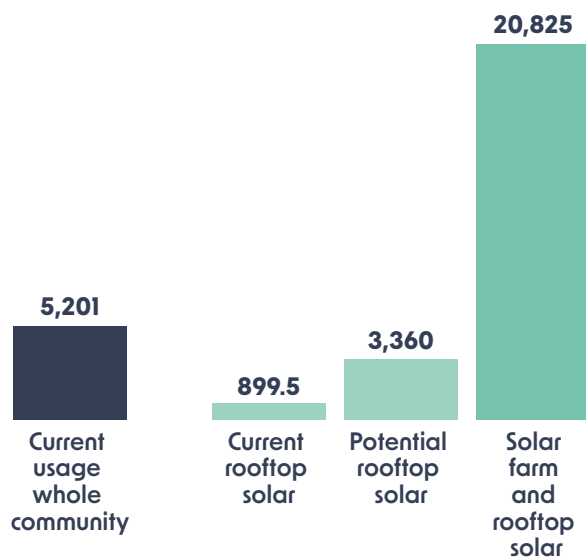
Figure 1 The Tilba's solar and microgrid potential supply (kWh/day)
